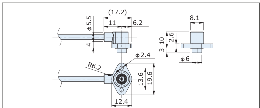
Right Angle Plug CRS9001-3101F
